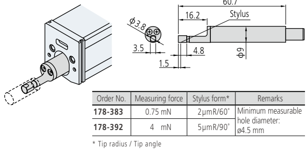
Small Hole Detectors
