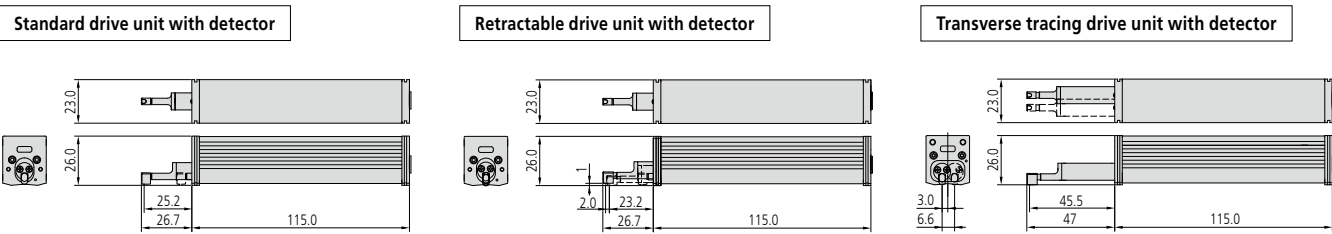
Drive unit attached with detector
