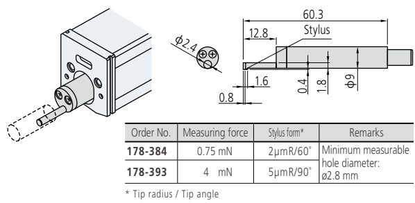
Extra Small Hole Detectors
