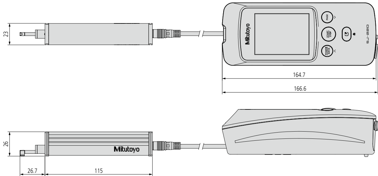
Drive unit not stored inside display unit (Standard detector installed in drive unit)
