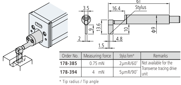
Deep Groove Detectors
