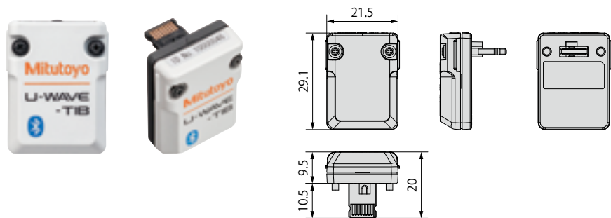
Wireless Unit for Measuring Instrument U-WAVE-TIB
