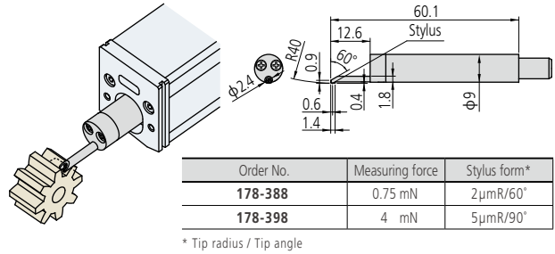
Gear-tooth Surface Detectors
